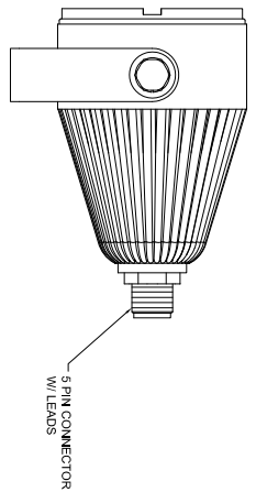
7030-36040-7 CAMERA CA 50 WATER TIGHT BLACK AND WHITE 3.6 MM. FORWARD VIEWING, HIGH RESOLUTION, 6000 LINES, 0.0003 LUX, 12 VDC @ 110mA WITH 5 PIN CONNECTOR
