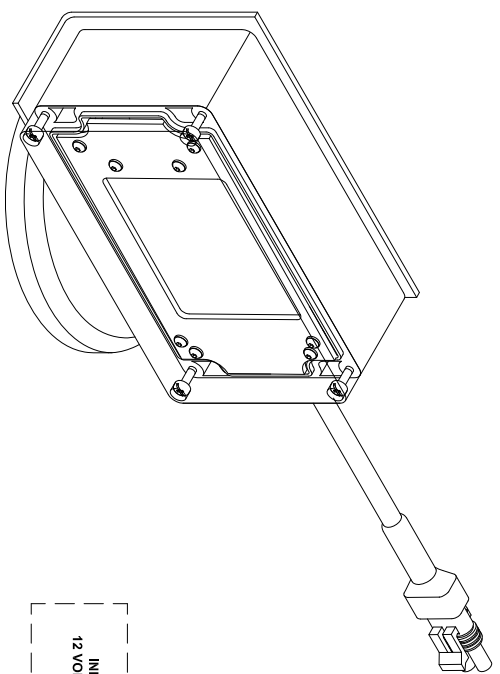
MODEL 7030-33665-60 RIGHT HAND CONNECTIONS SINGLE 4" LCD MONITOR ENCLOSURE 12 VOLT DC FOR UNDER GROUND USE WITH 5 PIN CONNECTORS
